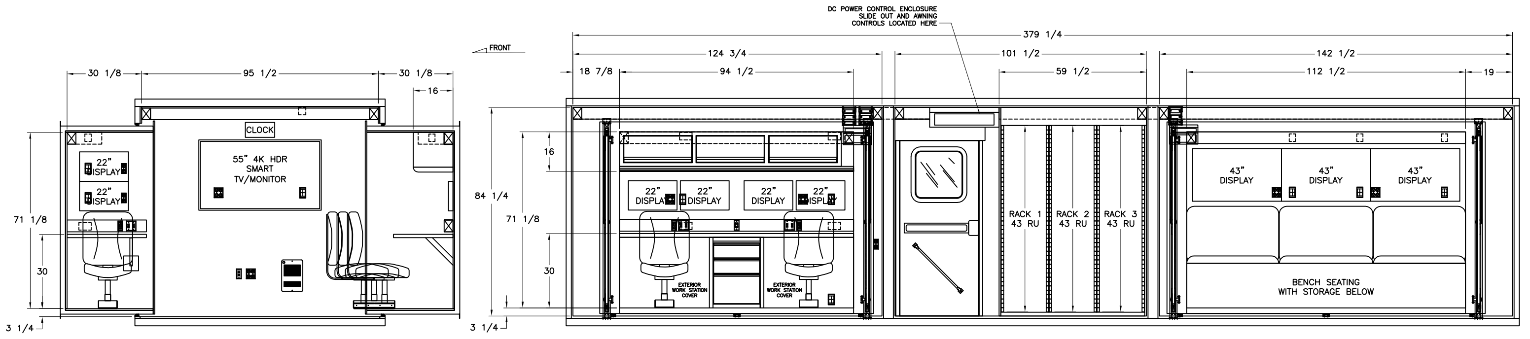
FRONT WALL INTERIOR LAYOUT
